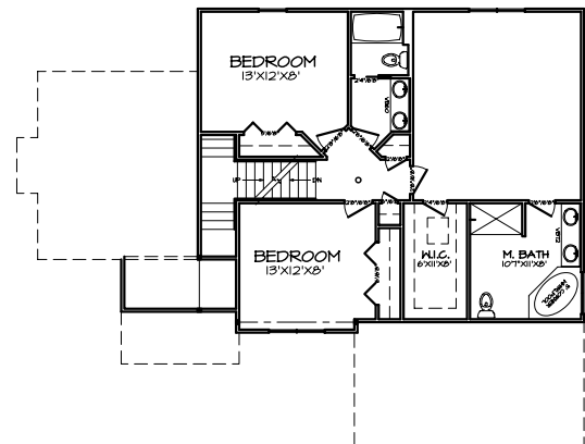
SECOND FLOOR PLAN A-3
