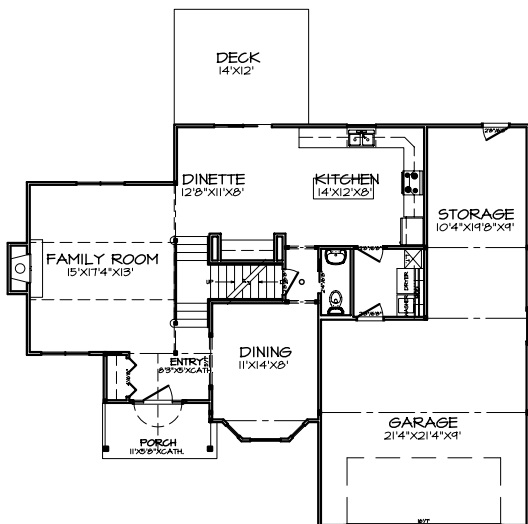
FIRST FLOOR PLAN A-2
