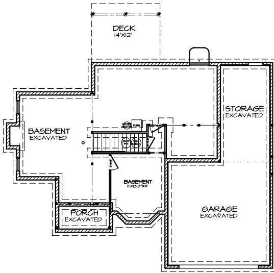
FOUNDATION PLAN A-3
